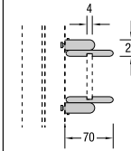
M 1580 Panel retainer with slot
